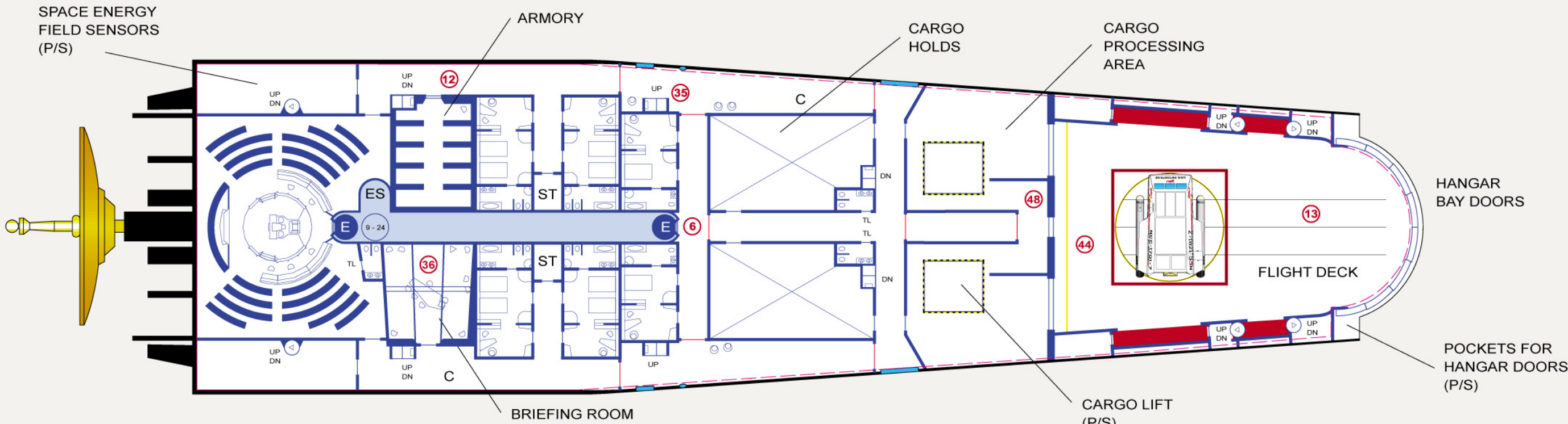
DECK 19 (H DECK): SECONDARY BRIDGE / HANGAR DECK DECK 11 (Secondary Hull)
